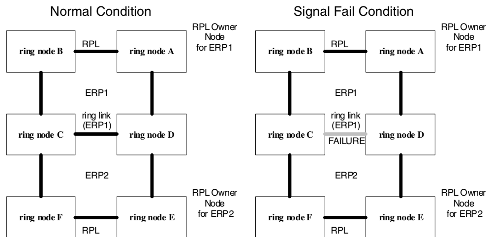
Figure 312: Ring Interconnection Architecture (Multi-ring/Ladder Network)
