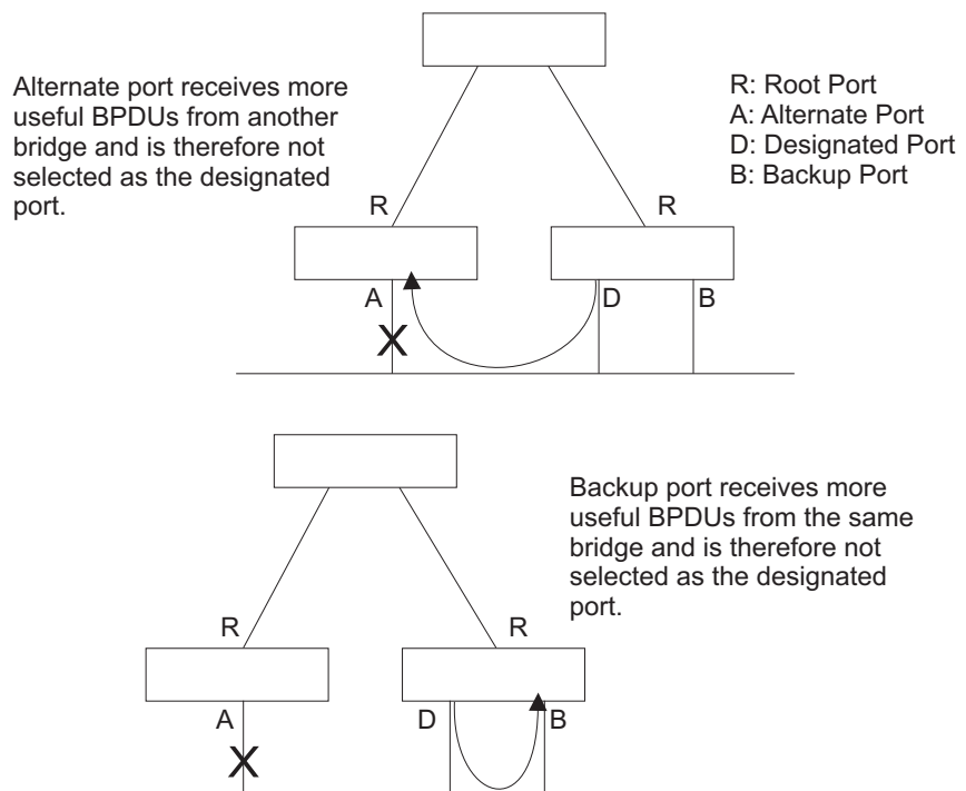
Figure 126: STA Port Roles
