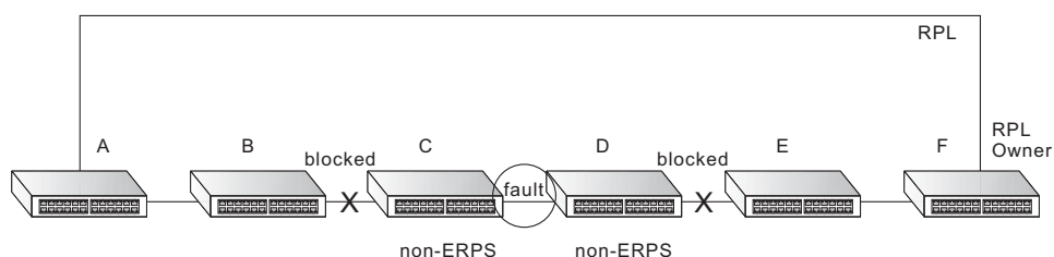
Figure 316: Non-ERPS Device Protection
