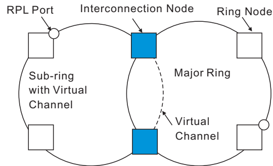
Figure 314: Sub-ring with Virtual Channel
