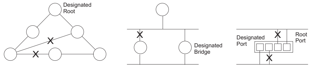
Figure 116: STP Root Ports and Designated Ports
