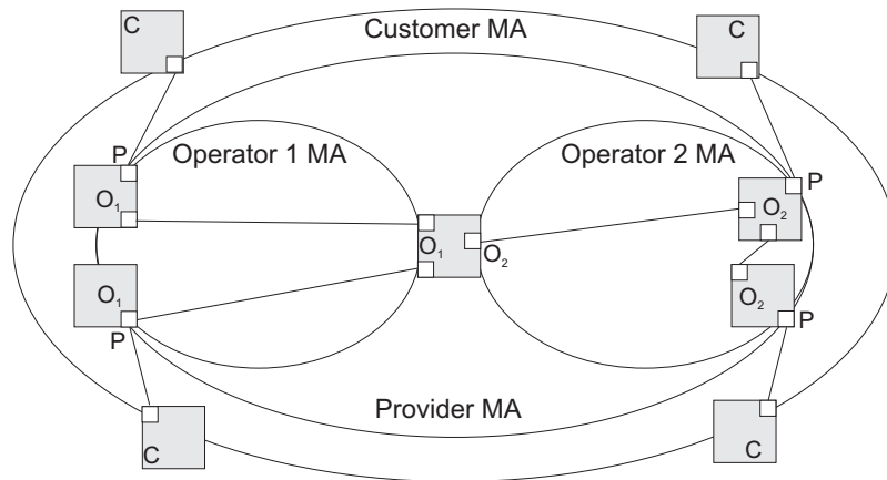
Figure 328: Multiple CFM Maintenance Domains
