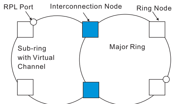
Figure 315: Sub-ring without Virtual Channel
