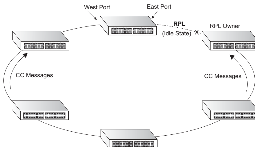
Figure 311: ERPS Ring Components
